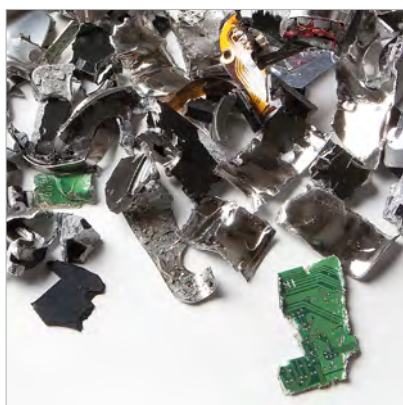
Particles of shredded hard drives Cutting size: 20 x 40-50 (<1000 m²). Security level: H-4
