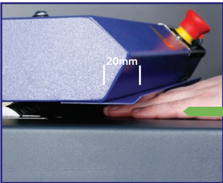
Additional 20mm safety guard fitted to all Optimax Ecopax Shredders
